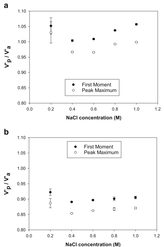
Fig. 6 Retention ratios for lysozyme injections on a Toyopearl AF-Formyl column (a) and on a Toyopearl AF-Amino column (b) as a function of NaCl concentrations (20 mM sodium acetate pH 4.5).
